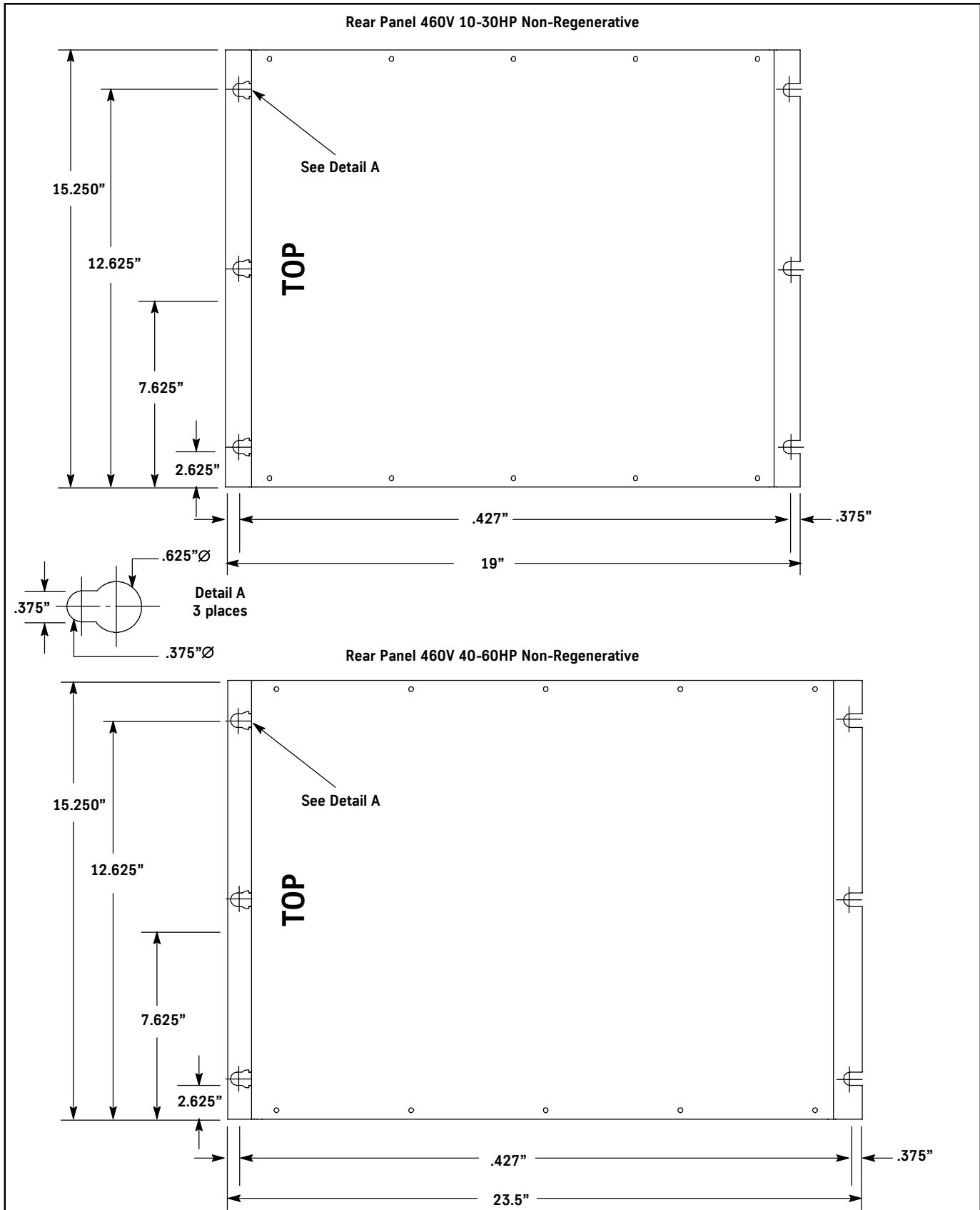
Figure 5 - Mounting Specifications
