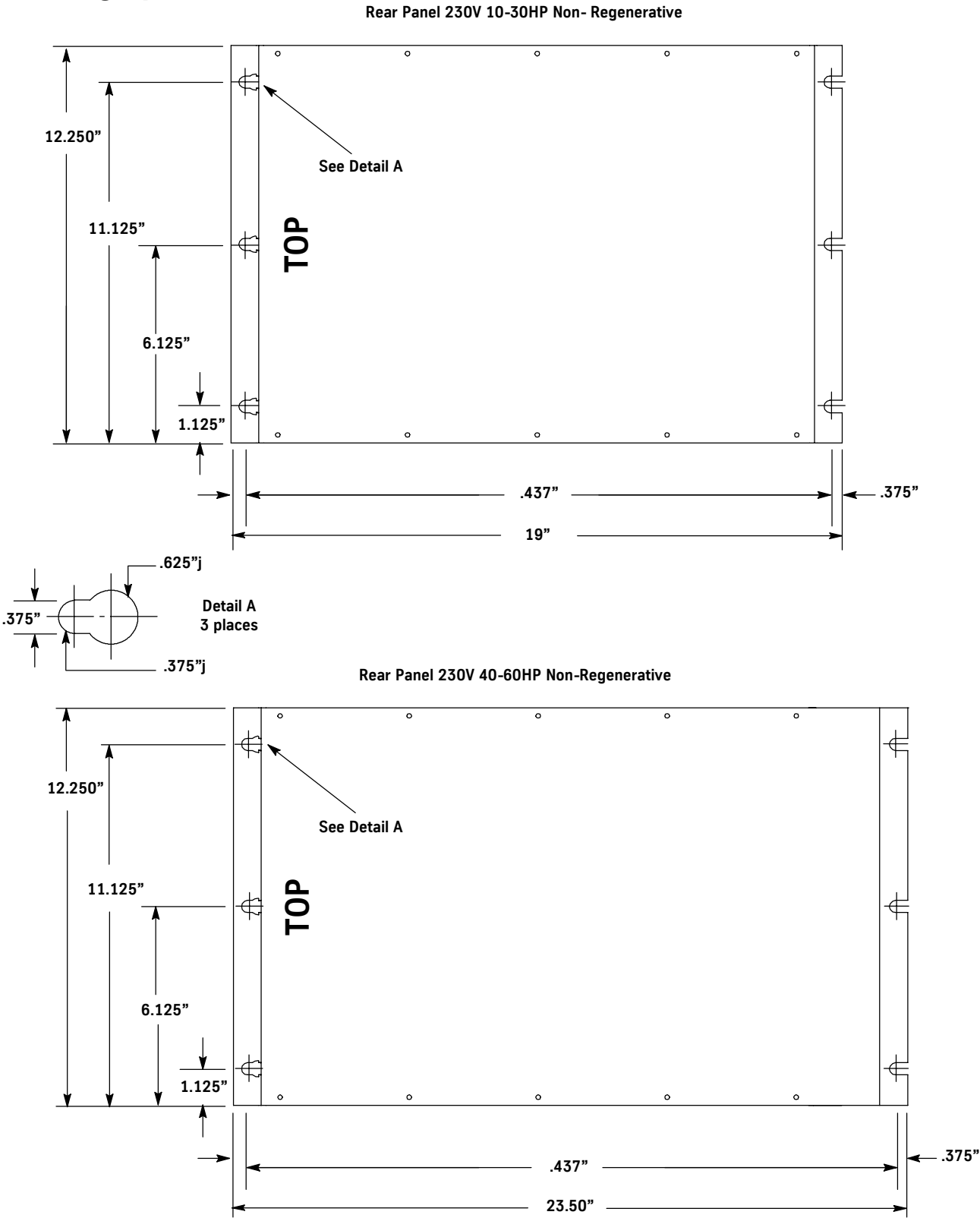
Figure 4 - Mounting Specifications
