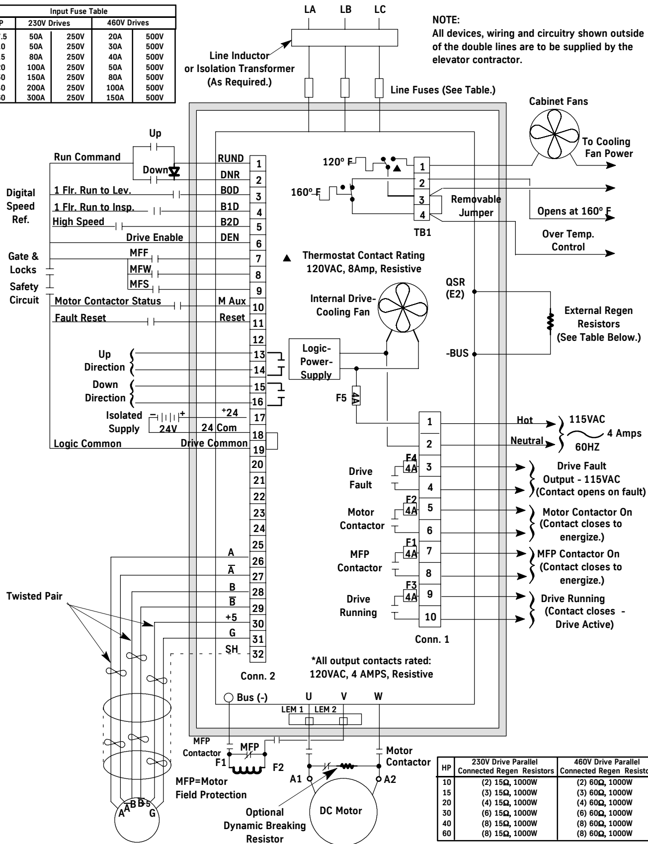
Figure 24 - Non-Regenerative Drive Interface Wiring (Digital Speed Pattern-DC)
