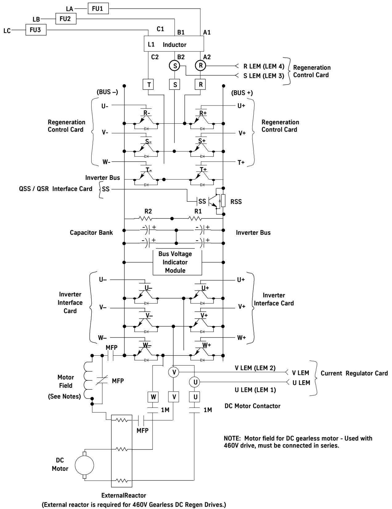
Figure 30 - Quantum Quiet Regenerative DC Drive
