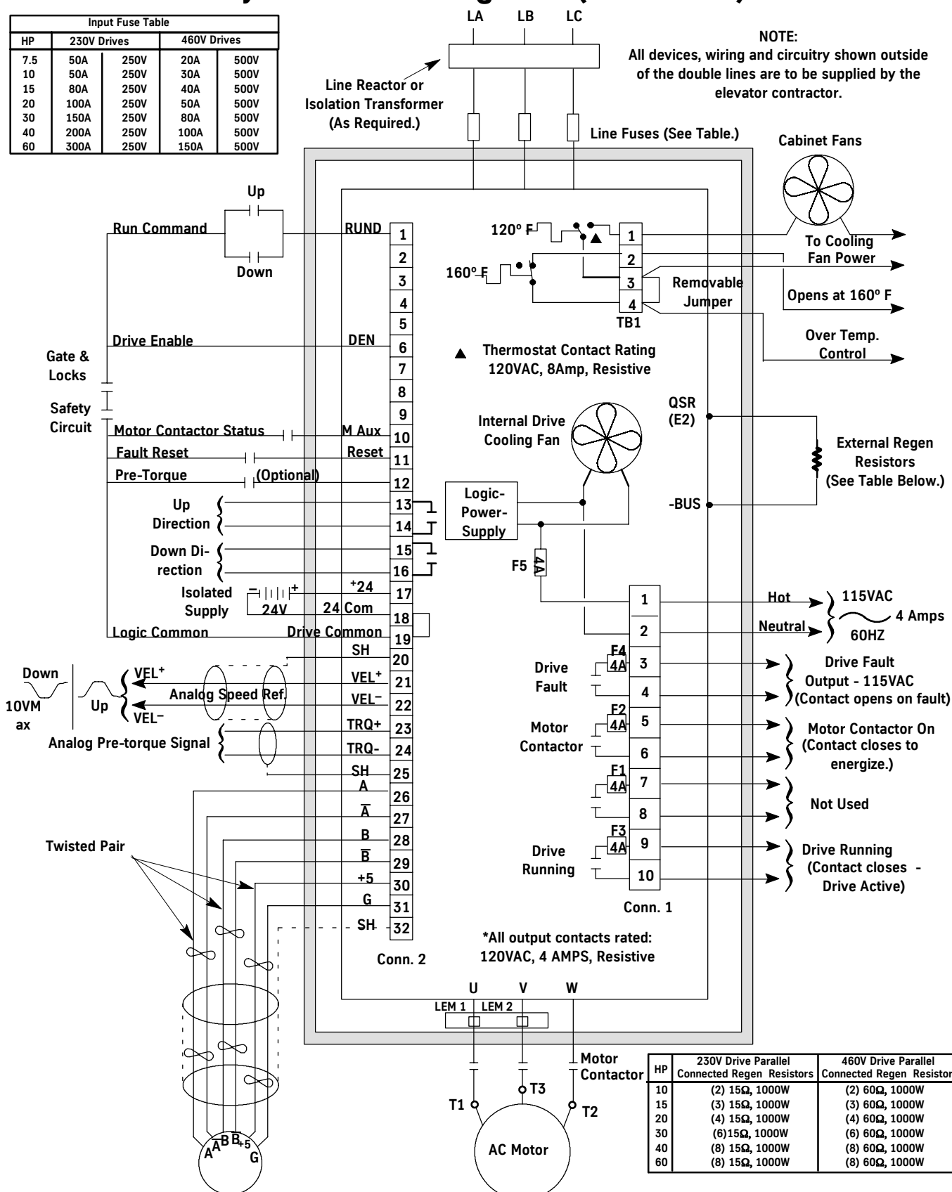
Figure 21 - Non-Regenerative Drive Interface Wiring (Analog Speed Pattern - AC)
