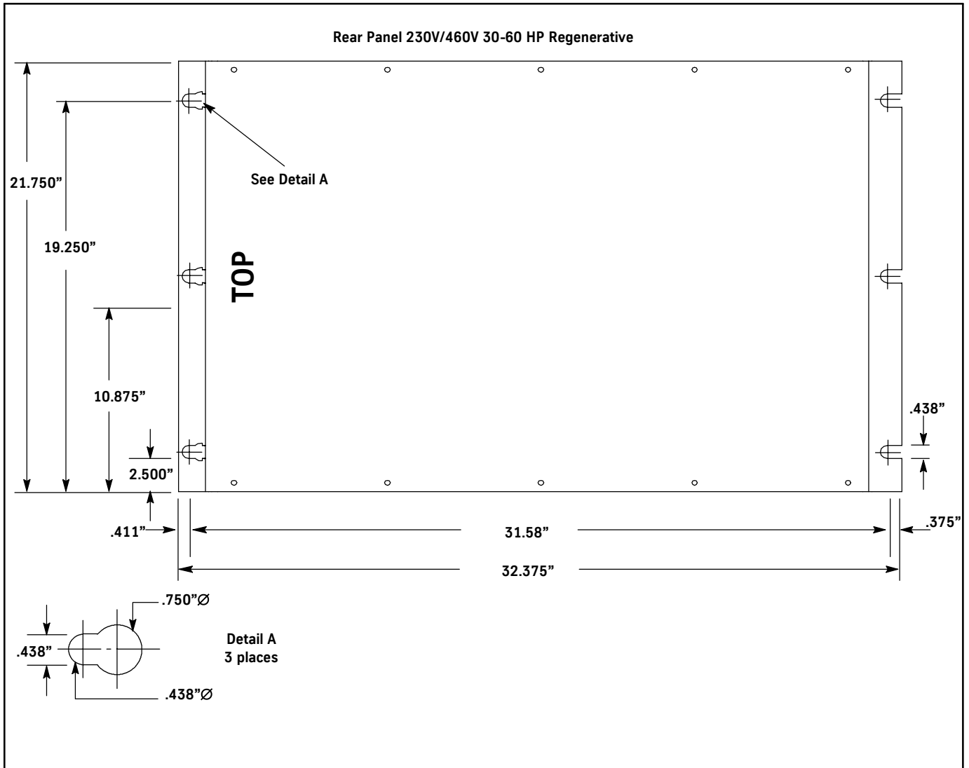
Figure 6 - Mounting Specifications
