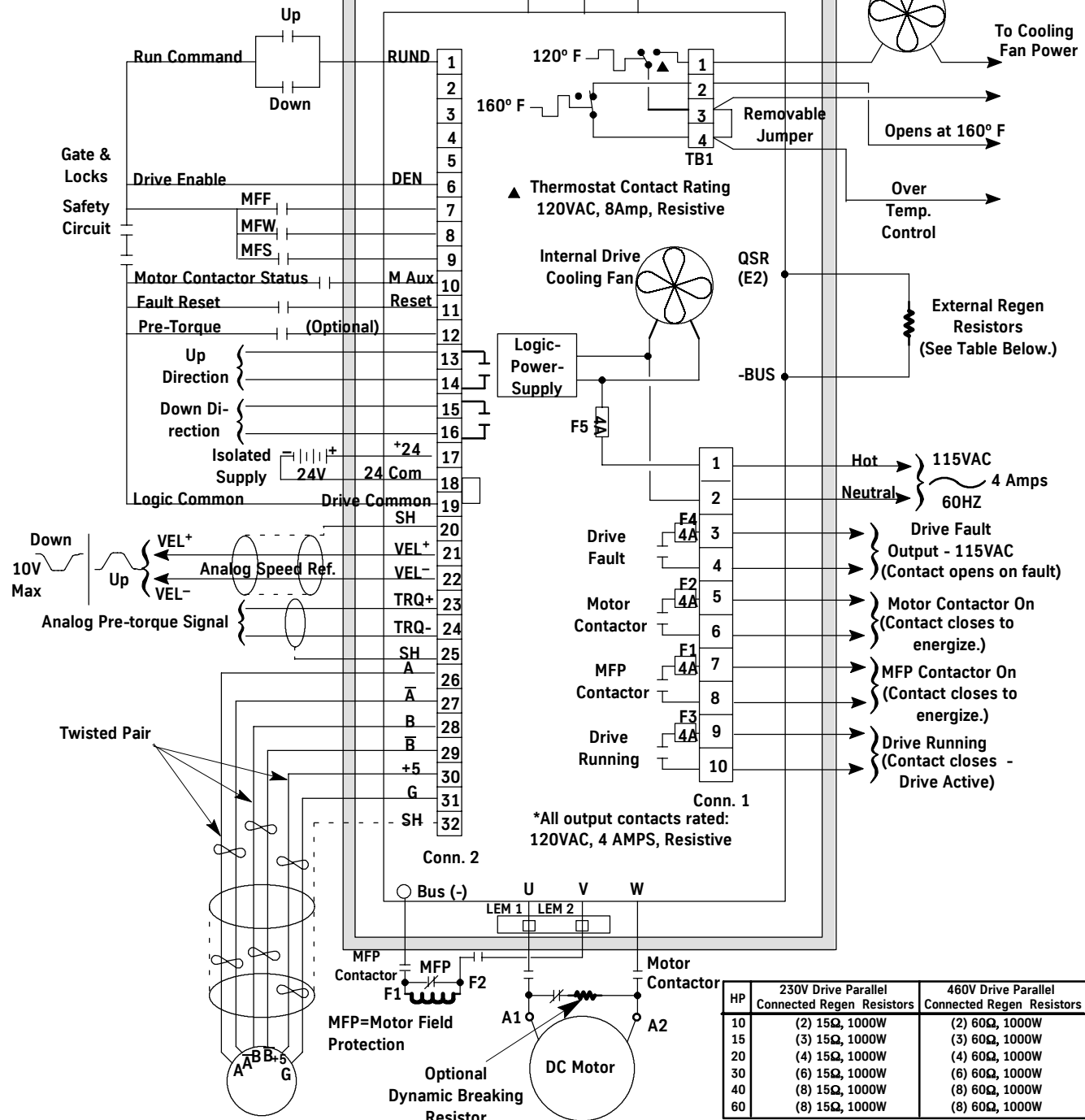
Figure 23 - Non-Regenerative Drive Interface Wiring (Analog Speed Pattern - DC)
