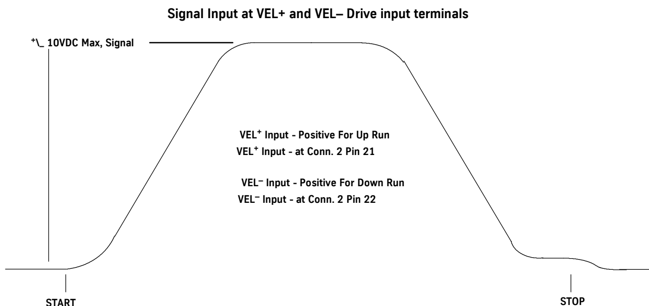
Figure 18 - Analog Speed Pattern (S-Curve), Signal
