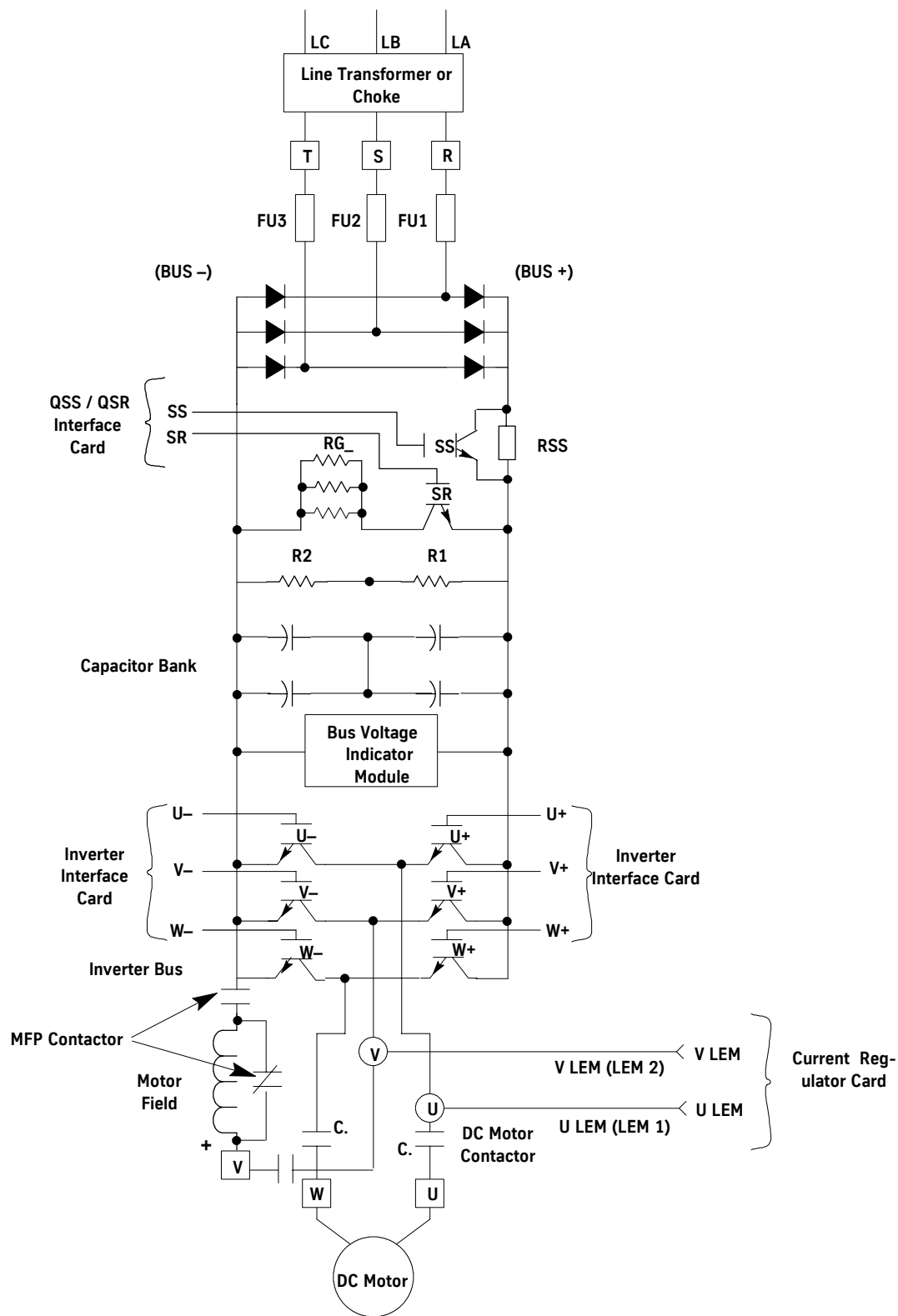
Figure 28 - Quantum Quiet DC Drive (Non-Regenerative)
