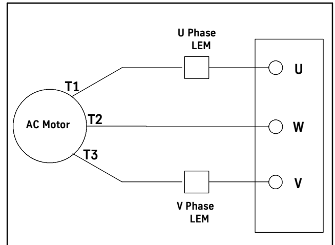
Figure 11 - AC Output Wiring without Motor Contactor
